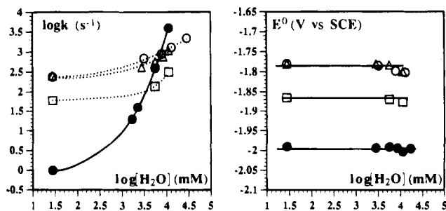
Figure 4. Variation of the cleavage rate constant and of the standard potential of the anion radical with water concentration in compounds of group B \text{CH}_3\text{CN} + 0.1 \text{ M } n\text{-Bu}_4\text{NBF}_4 . (○) 4a , (△) 4b , (□) 5 , and (●) anthracene.
