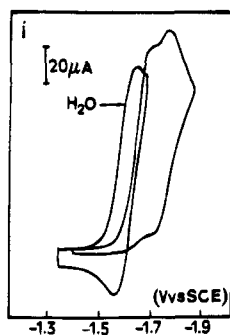
Figure 1. Cyclic voltammety of 1 (2 mM) in \text{CH}_3\text{CN} + 0.1 \text{ M } n\text{-Bu}_4\text{NBF}_4 in the presence and absence of water (0.58 M). Scan rate: 0.2 V/s.
