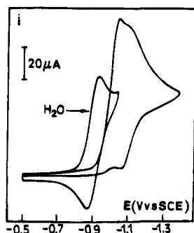
Figure 2. Cyclic voltammety of 2a (2 mM) in \text{CH}_3\text{CN} + 0.1 \text{ M } n\text{-Bu}_4\text{NBF}_4 in the presence and absence of water (2.6 M). Scan rate: 0.5 V/s.
