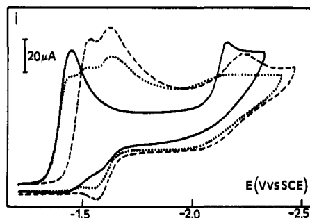
Figure 9. Cyclic voltammetry of 1 (1.85 mM) in DMF + 0.1 M n\text{-Bu}_4\text{NBF}_4 in the absence (—) and in the presence of 0.5 mM (···) and 1 mM (---) \text{Mg}(\text{ClO}_4) . Scan rate: 0.5 V/s.
