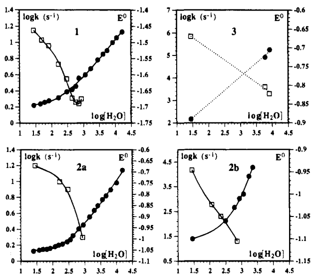
Figure 3. Variation of the cleavage rate constant and of the standard potential of the anion radical in compounds of group A in \text{CH}_3\text{CN} + 0.1 \text{ M } n\text{-Bu}_4\text{NBF}_4 . [\text{H}_2\text{O}] in mM and E^0 in V vs SCE.
